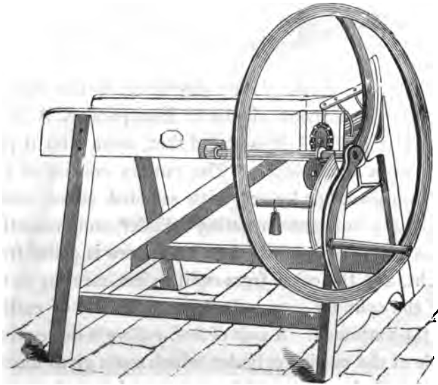
HEPPENSTALL'S CHAFF-ENGINE.
